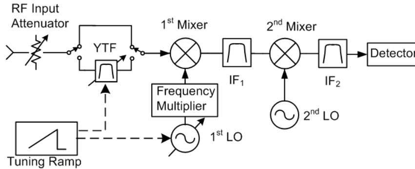
Figure 3-4. Highband Structure Block Diagram.
