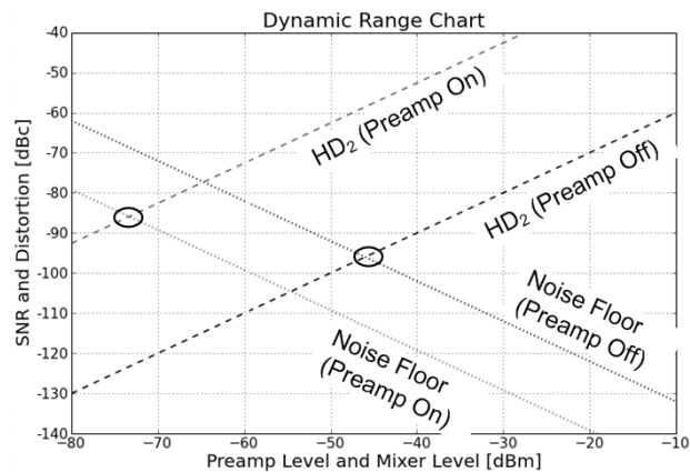
Figure 6-34. Preamp 2nd Harmonic Distortion and the Dynamic Range Chart
