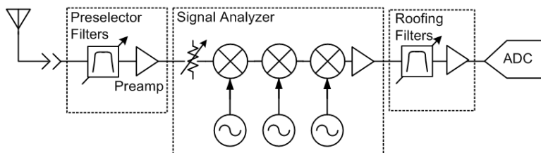
Figure 8-4. Spectrum Monitoring Receiver Block Diagram.
