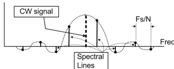
Figure 5-14. Spectrum of CW Signal with Spectral Leakage.
