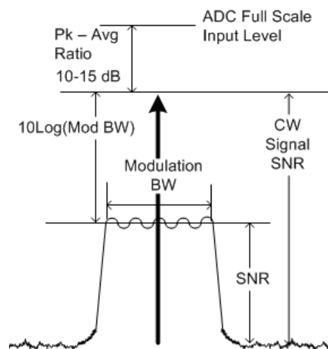
Figure 6-51. SNR of the Digitally Modulated Signal
