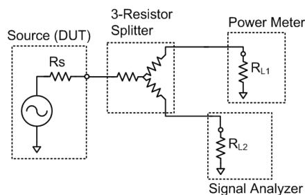
Figure 7-20. 3-Resistor Splitter.
