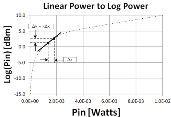
Figure 7-14. Small Value Amplitude Changes on the Log Scale are Approximately Linear.
