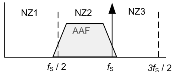
Figure 3-9. Bandpass Sampling in the Frequency Domain
