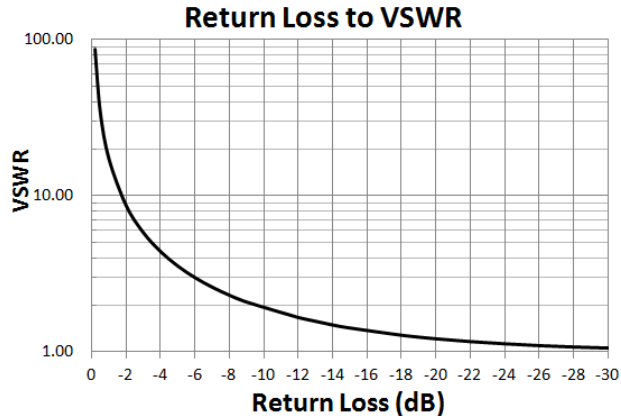
Figure 7-12. VSWR to Return Loss
