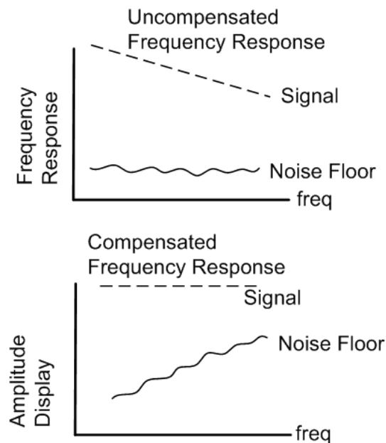
Figure 4-3. Frequency Response Compensation
