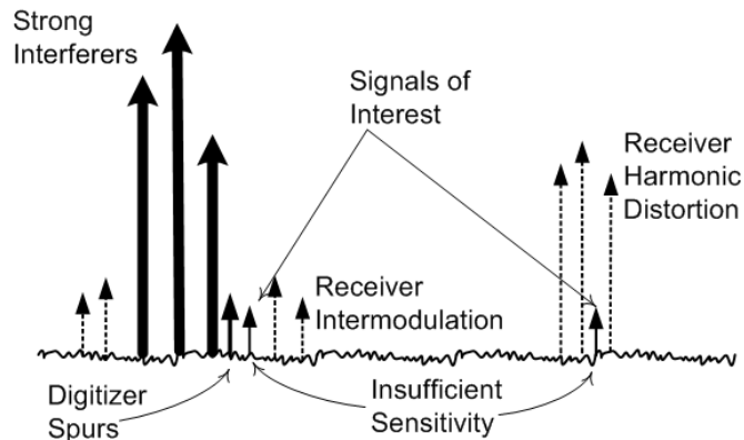
Figure 8-3. Distortion Created in the Signal Analyzer for the Spectrum Monitoring Situation.
