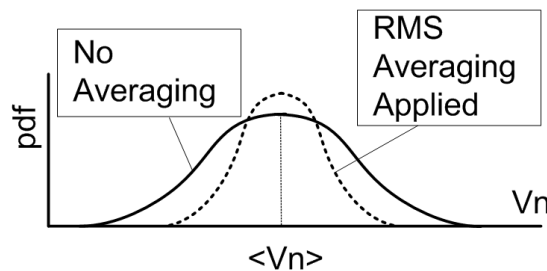
Figure 5-29. Variance Reduction with RMS Averaging
