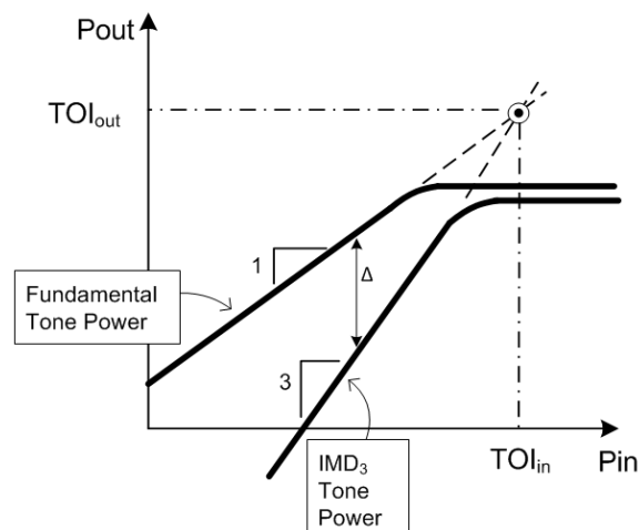
Figure 6-15. Third Order Intercept Point
