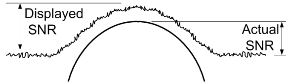
Figure 7-5. Near Noise Displayed SNR and Actual SNR.
