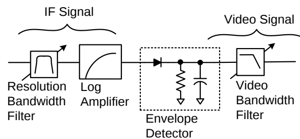
Figure 5-1. Analog IF Block Diagram
