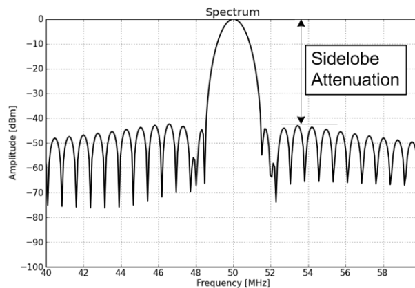
Figure 5-25. Hamming Widowing Function Sidelobe Attenuation
