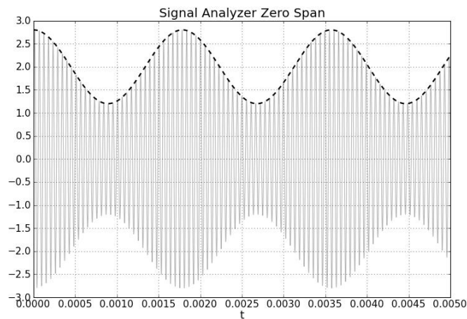
Figure 5-8. Amplitude Modulation in the Time Domain.
