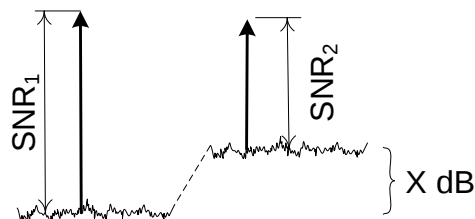
Figure 4-5. Display Adjusted for RF Input Attenuator Setting.
