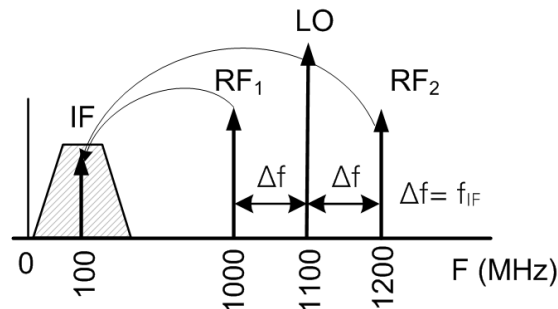
Figure 2-7. Desired Signal and its Image Response.
