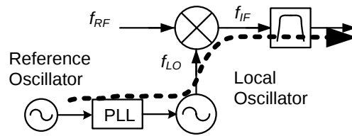
Figure 2-16. Residual Responses
