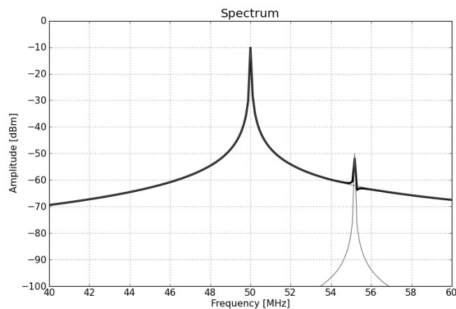
Figure 5-16. Spectral Leakage Masking a Nearby Signal.
