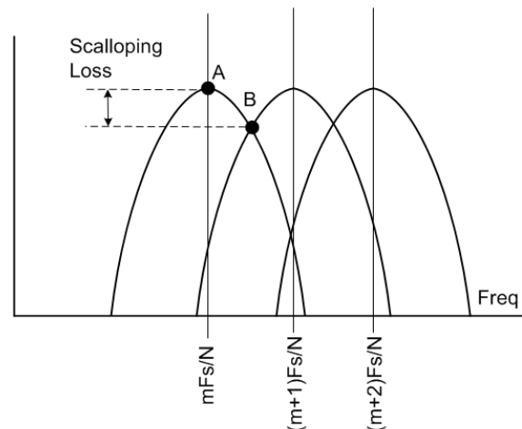
Figure 5-24. Scalloping Loss
